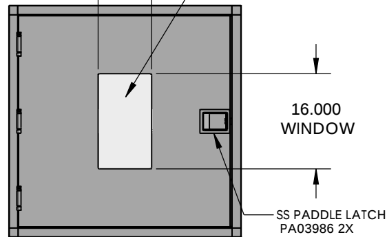
FRONT VIEW (CLEAN ROOM SIDE)
